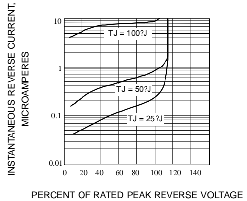
Fig. 4-TYPICAL REVERSE CHARACTERISTICS
